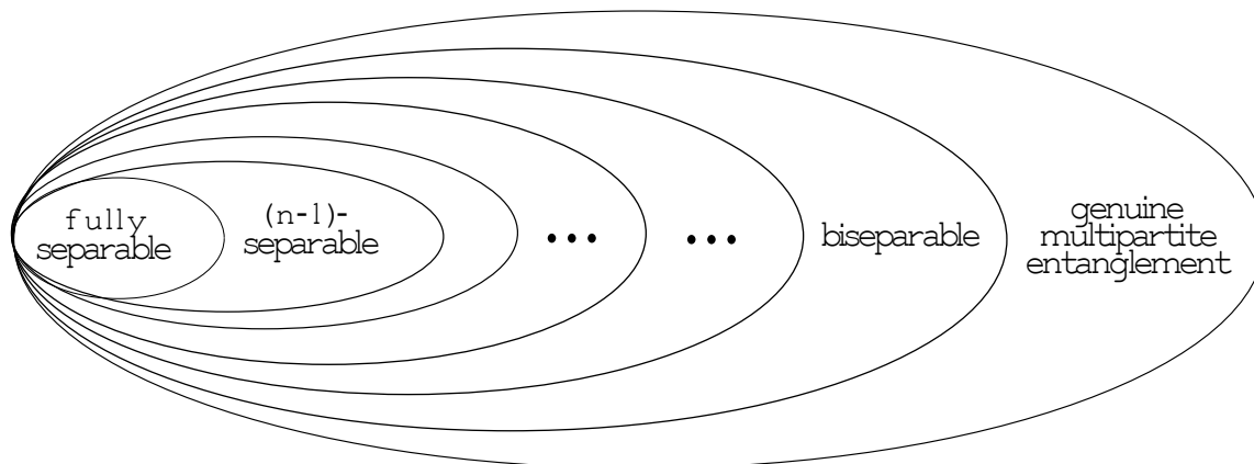
Figure 4.1: Schematic illustration of the structure of the different sets of states, from fully separable to genuine multipartite entangled. [56]
