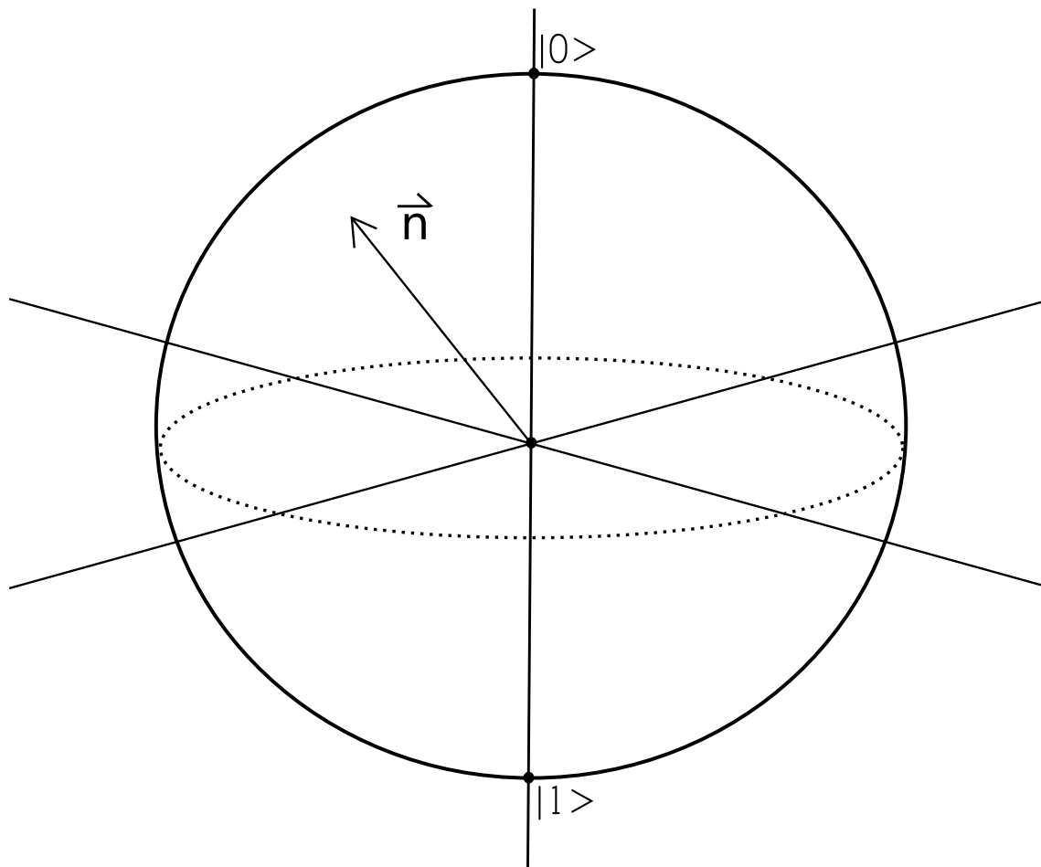
Figure 3.1: Bloch picture: The state space of all possible qubit states can be represented by the Bloch ball, which is formed by all possible Bloch vectors \vec{n} . [56]
