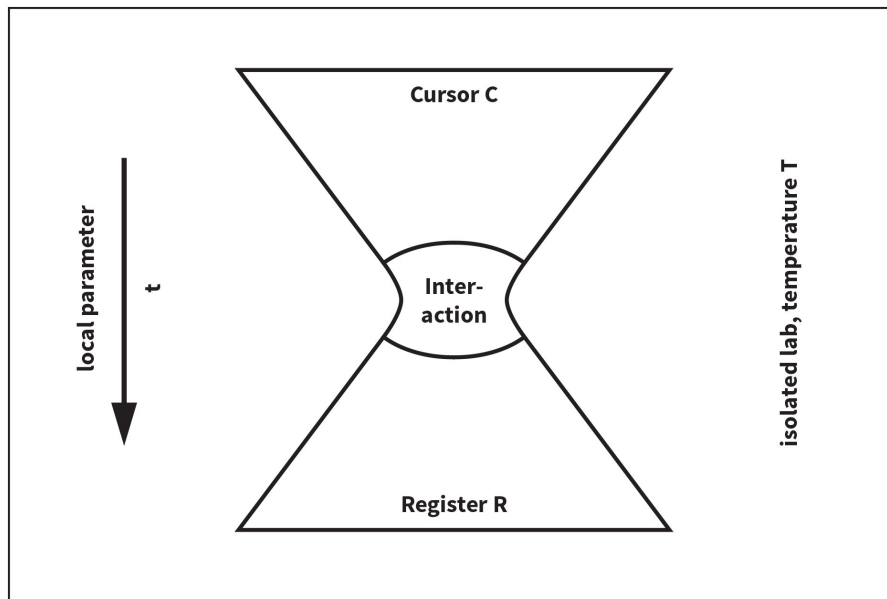
Figure 6.1: Schematic illustration of the Quantum Hourglass [198].
