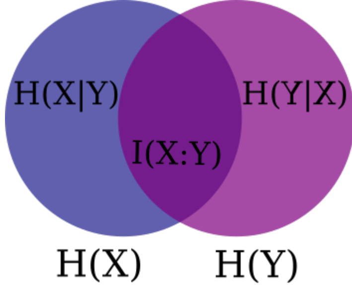
Figure 2.1: Venn diagram of the Shannon entropies of a bipartite system [56].
