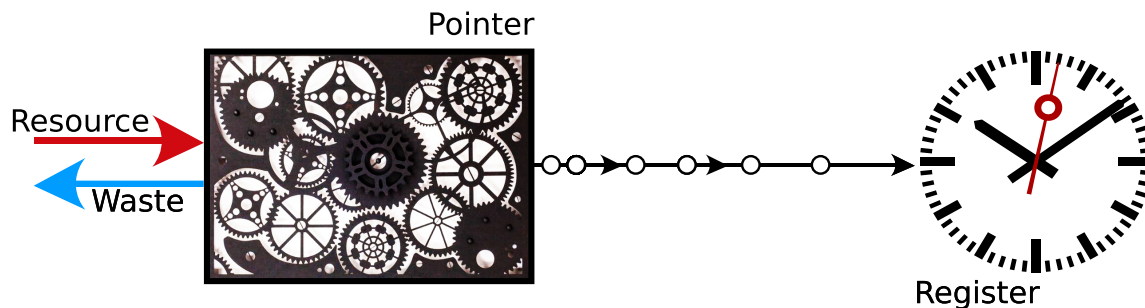
Figure 6.2: A pointer system generates a sequence of events that are recorded by the register [56].
