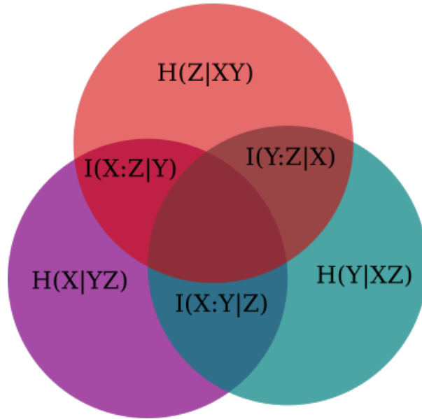
Figure 2.2: Venn diagram of the conditional Shannon entropies of a tripartite system [56].
