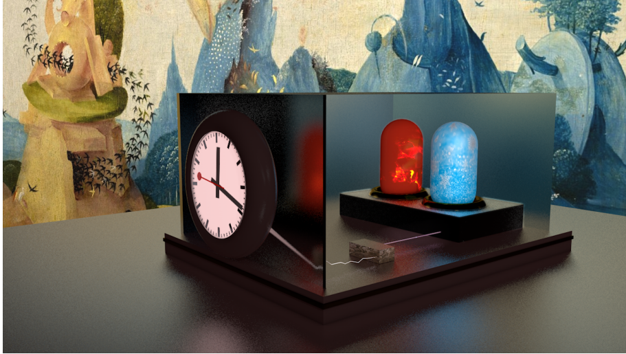
Figure 6.4: Creative illustration of the minimal thermal clock [56].
